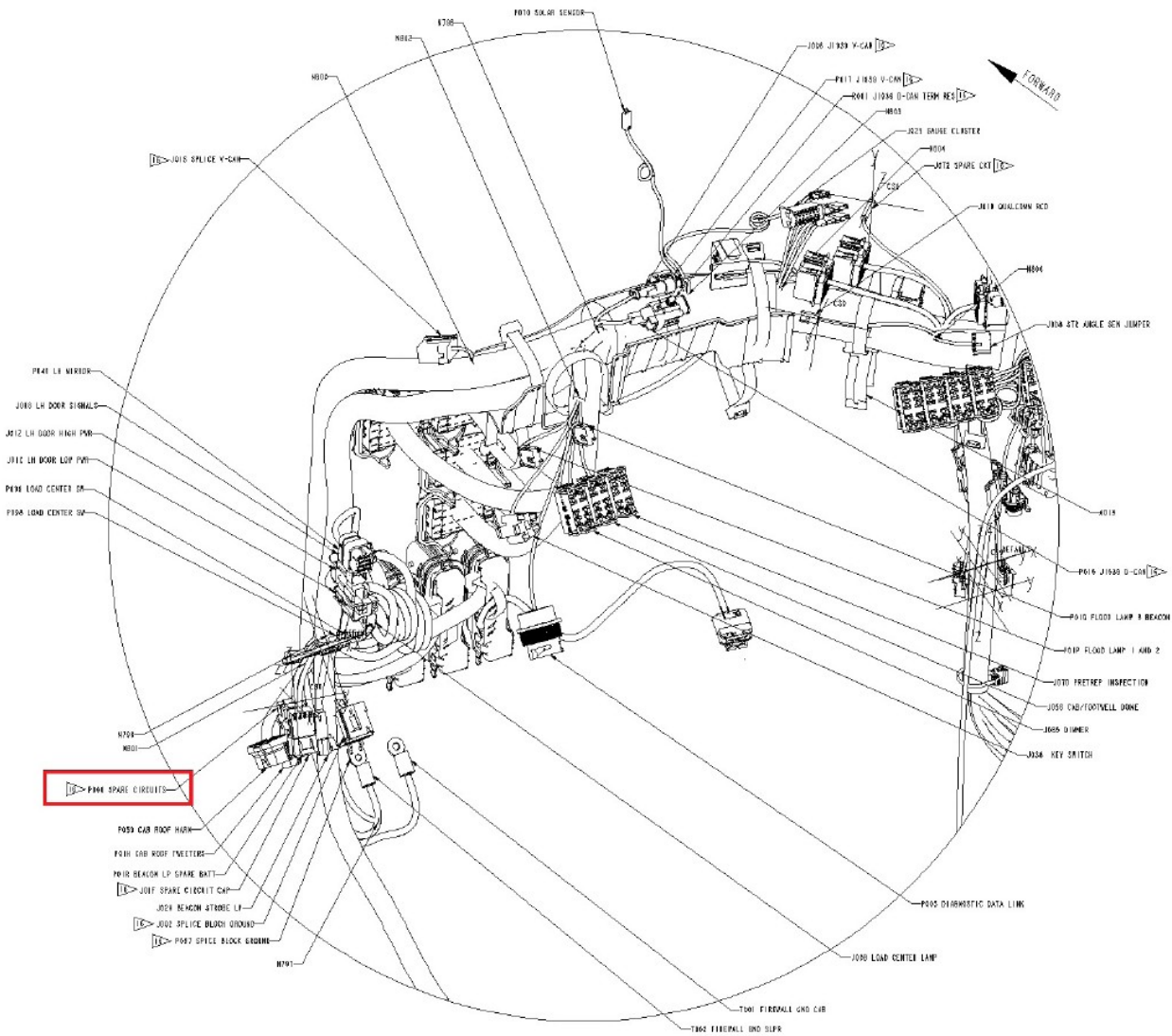
Spare Circuit Connector and Pinout Details
