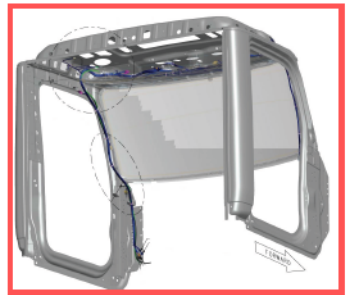
CAB ROOF HARNESS 1) Connections to Main Cab IP Harness 2) Connections to Antennas 3) Connections to Roof Lighting
