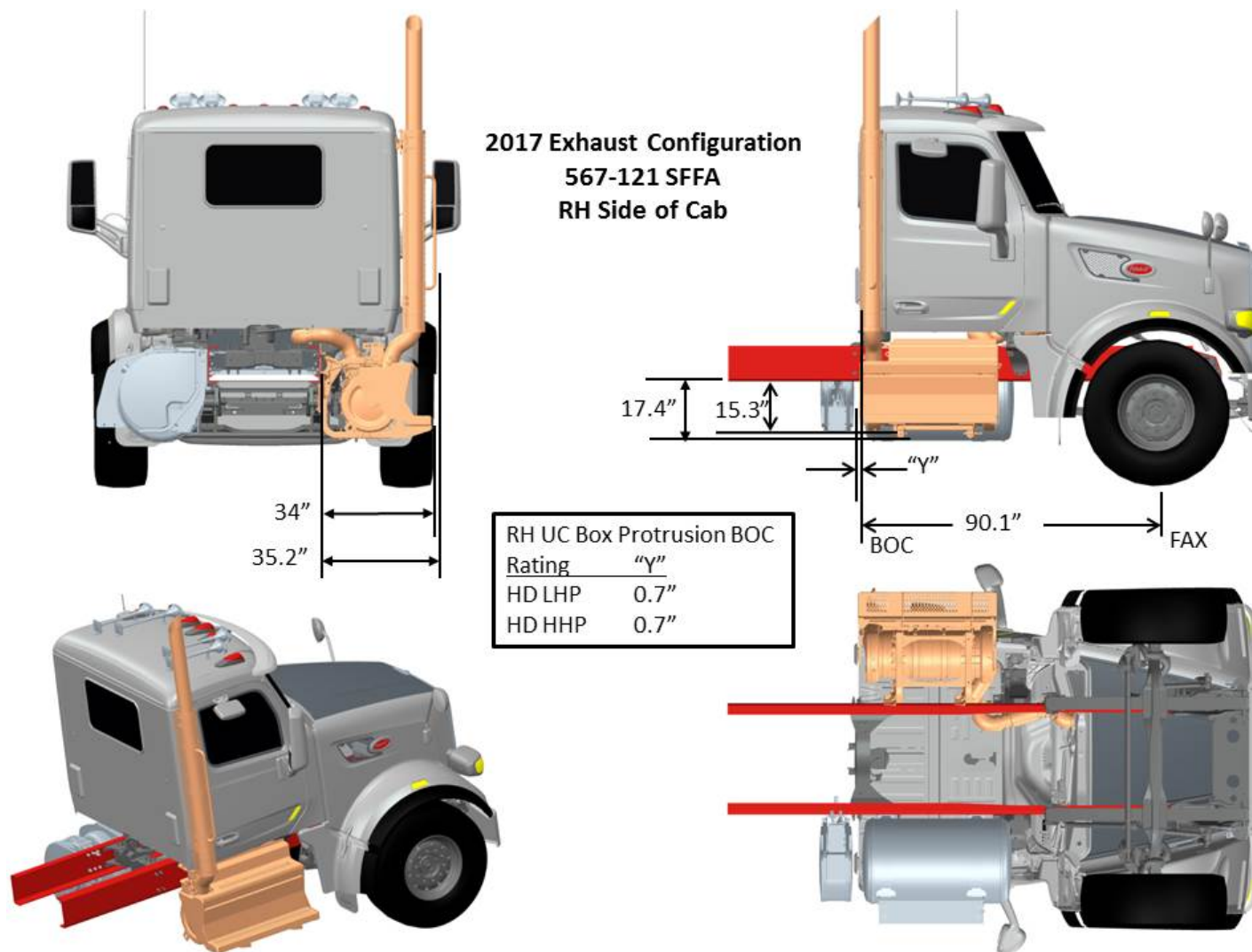
FIGURE 3-92. Exhaust Single RH Side of Cab DPF/SCR RH Under Cab
