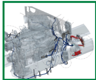
ENGINE HARNESS 1) Connections to Main Chassis Harness 2) Connections to Firewall Bulkhead 3) Connections to Starter 4) Connections to Aftertreatment Harness 5) Connection to Engine ECU
