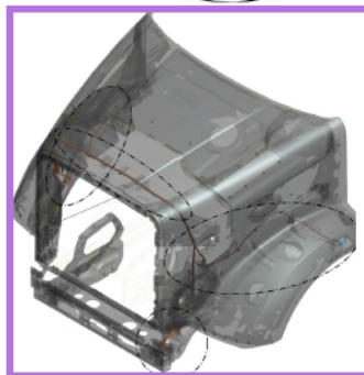
HOOD CHASSIS HARNESS 1) Connections to Main Chassis Harness 2) Connections to Head Lights 3) Connections to Turn Signal Lamps
