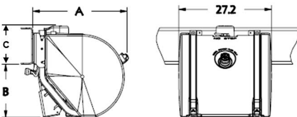
FIGURE 3-40. DEF Tanks
