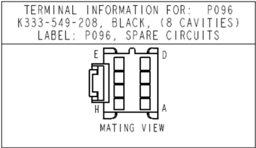
Spare Circuit Connector and Pinout Details
