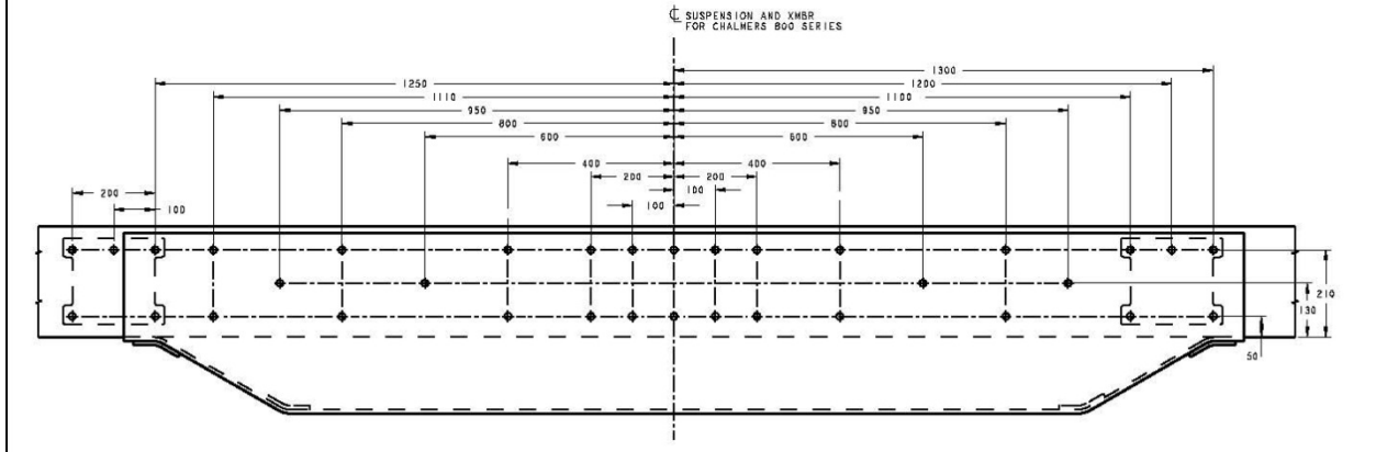
FIGURE 3-31. Chalmers Tandem Suspension Guppy
