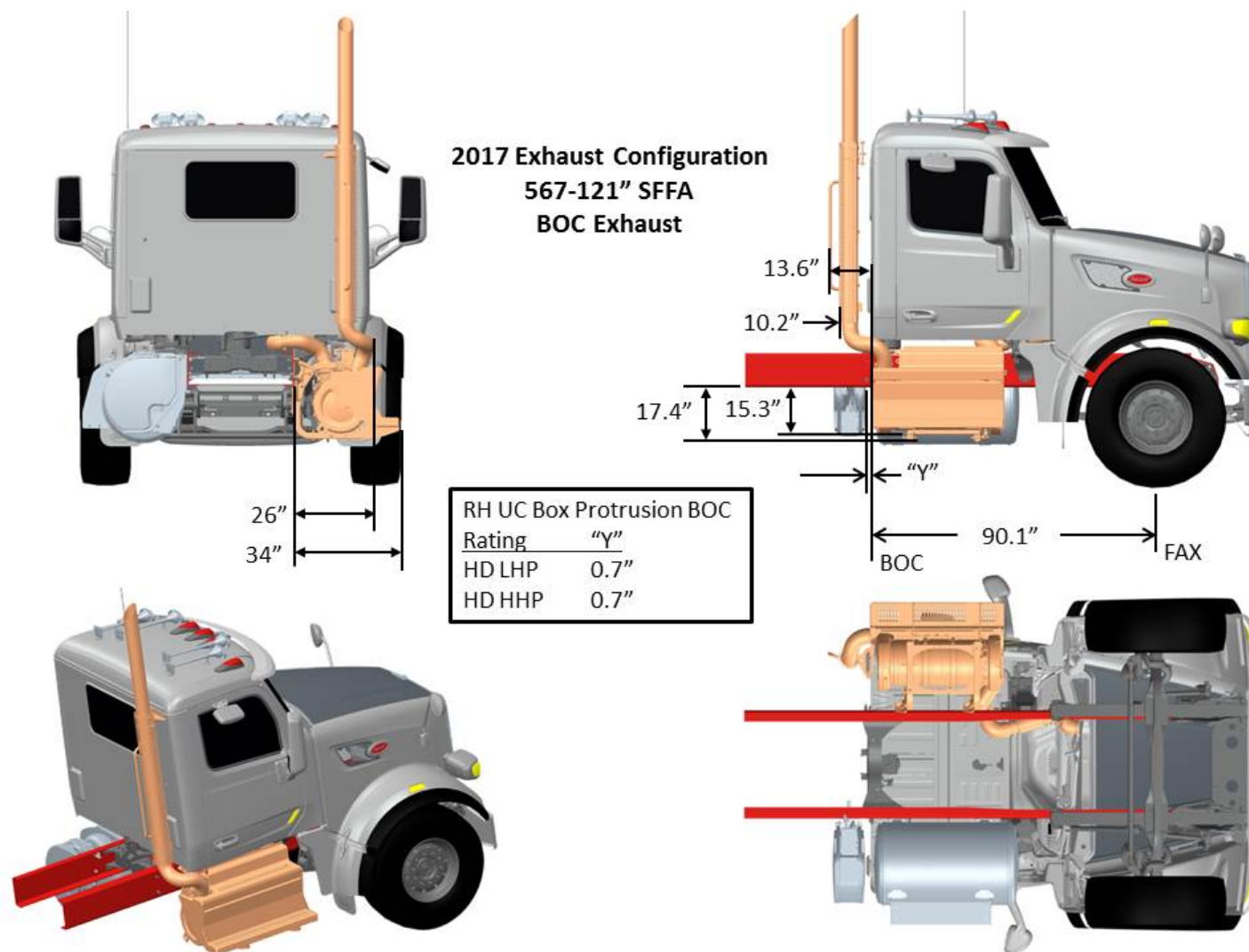
FIGURE 3-91. Exhaust Single RH Back of Cab DPF/SCR RH Under Cab
