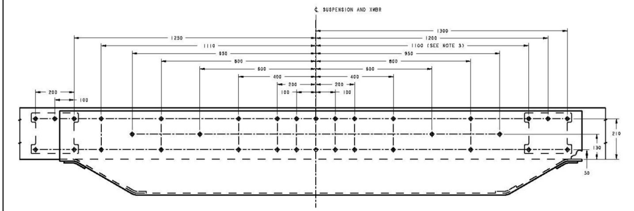
FIGURE 3-32. Hendrickson HN/HMX/R Tandem Suspension Guppy
