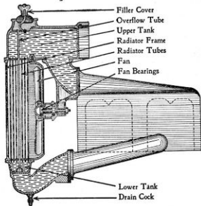
Figure 129.—Cooling System of the Fordson Tractor.
