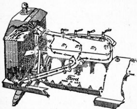
Figure 24.—The Water Cooling System.
