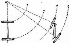
Figure 42.—Action of Steering Gear.
