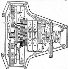
Figure 83.—Transmission. A, B, C—Magneto Support, Coils and Magnets; D—Flywheel; E—Triple Gears; F, G—Reverse and Low Speed Bands; H—Clutch; I—Brake Band.
