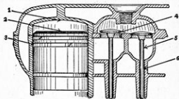
Figure 59.—Carbon Deposit. 1—Combustion Space, 2—Piston Head, 3—Ring Grooves, 4—Valve Face, 5—6—Valve Stem.
