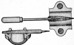
Figure 76.—Drawfiling (left) and Scraping (right).
