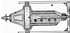
Figure 10.—Three Point Engine Mounting.
