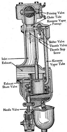
Figure 134.—End View of Vaporizer.
