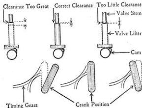
Figure 67.—Effect of Various Amounts of Valve Clearance.
