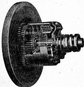
Figure 26.—The Transmission and High Speed Clutch.
