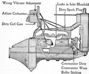
Figure 94.—General Troubles Causing Loss of Power.
