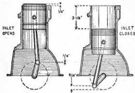
Figure 65.—Measurements for Inlet Valve Timing.
