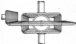
Figure 33.—Operating Principle of the Differential.
