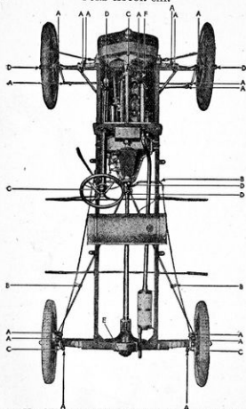
Figure 55.—Oiling Chart for the Ford Car: A, Oil Every 200 Miles; E, Oil Every 500 Miles; C, Grease Every 200 Miles; D, Grease Every 400 Miles; E, Grease Every 1,200 Miles; F, Oil Motor Daily; G, Grease Every 5,000 Miles.
