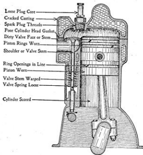
Figure 62.—Points of Compression Loss.
