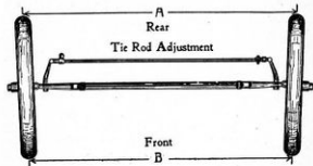
Figure 38.—Front Wheel Setting.
