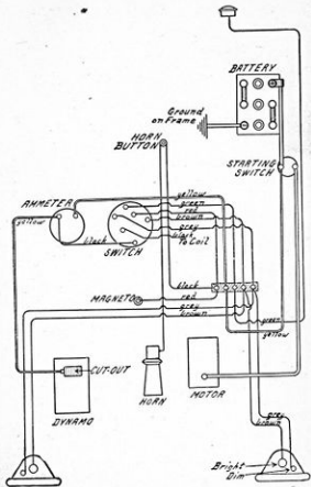
Figure 111.—Wiring of Later Cars.
