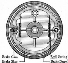
Figure 43.—Rear Wheel Emergency Brake.
