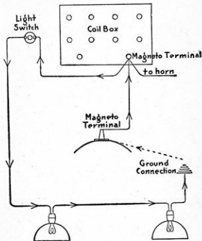
Figure 101.—Wiring of Ignition and Lighting System.
