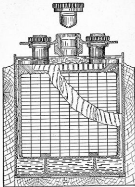
Figure 106.—Type of Battery Used With Ford Electric System.
