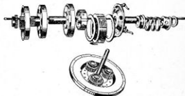
Figure 82.—Transmission Ready for Assembling.
