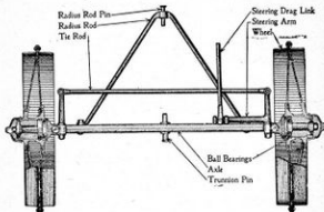
Figure 138.—Front Axle and Steering Rods.
