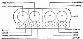
Figure 66.—Firing Order of the Ford Engine.
