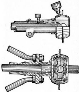
Figure 30.—The Universal Joint.
