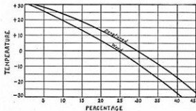
Figure 54.—Chart for Anti-Freeze Solutions.
