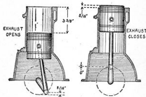
Figure 64.—Measurements for Exhaust Valve Timing.
