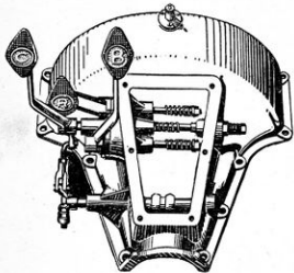
Figure 84.—Transmission Band Adjustments.
