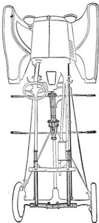
Figure 119.—Extended Ford Frame and Lengthened Shaft.
