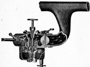
Figure 11.—The Ford Carburetor.
