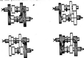
Figure 136.—Gear Positions. Upper Left—Low Gear. Lower Left—Intermediate. Upper Right—High Gear. Lower Right—Reverse.
