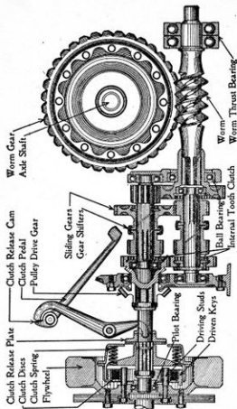
Figure 135.—Clutch, Transmission and Worm Drive of Tractor.
