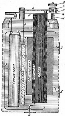
Figure 77.—Construction of Ford Coil Unit.
