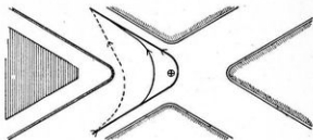
Figure 50.—Right and Wrong Way of Turning Sharp Corner.
