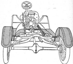
Figure 120.—Ford Frame Extended by Addition at Center. be used to make a motor truck having a load carrying capacity of from 1,000 pounds to 1½ tons.
