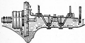
23.—The Ford Oiling System.
