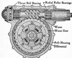
Figure 116.—Worm Drive of Ford Truck Rear Axle.
