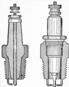
Figure 19.—One- and Two-Piece Spark Plugs.
