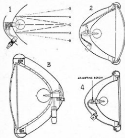
Figure 108.—Focusing Adjustments: 1—Correct and Incorrect Paths for Light Rays (A, Correct; B or C, Incorrect). 2—Adjusting Screw Above Reflector. 3—Adjustment in Lamp Housing. 4—Adjustment in Socket.
