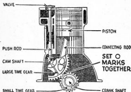
Figure 68.—Setting the Timing Gears.
