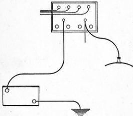
Figure 21.—Using a Battery With the Ford Ignition System.
