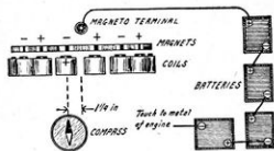
Figure 81.—Recharging Magnets in the Magneto.
