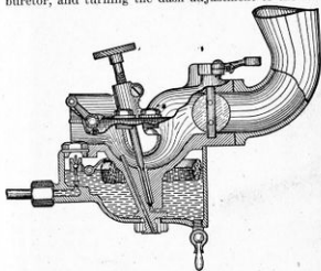
Figure 13.—Second Type of Ford Carburetor.
