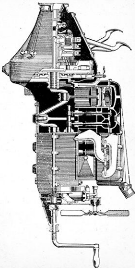
Figure 85.—The Ford Engine and Transmission.
