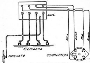
Figure 130.—Ignition Wiring Diagram.
