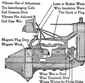
Figure 98.—General Ignition Troubles.
