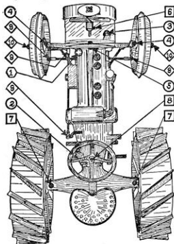
Figure 126.—Oiling Chart for Fordson Tractor.
