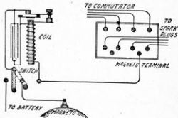
Figure 22.—Master Vibrator Connections.
