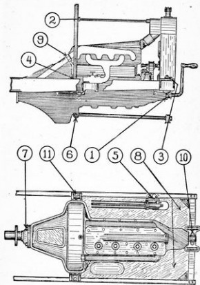
Figure 60.—Removing the Power Plant.
