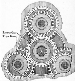
Figure 27.—The Triple Gears and Mounting.
