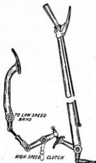
Figure 29.—High and Low Speed Controls.
