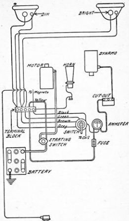
Figure 110.—Wiring of First Electrically Equipped Cars.
