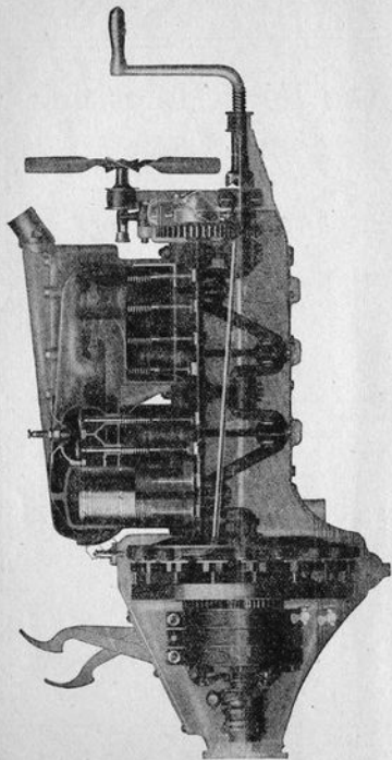
The Ford Power Plant.
