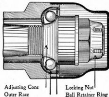
Figure 37.—Front Wheel Bearings.
