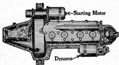
Figure 109.—Location of Ford Dynamo and Starting Motor.
