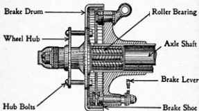
Figure 115.—Outer End of Truck Rear Axle.
