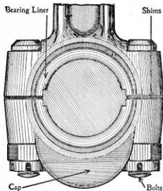
Figure 73.—Connecting Rod Bearing Fitted With Shims.
