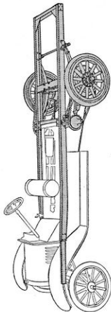
Figure 122.—Chain Driven Truck Unit.
