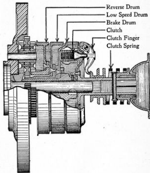
Figure 28.—The Transmission and Clutch.
