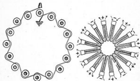
Figure 80.—Windings and Magnets of the Magneto.
