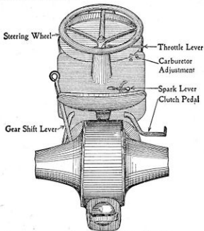
Figure 124.—Controls of the Tractor.
