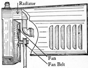
Figure 25.—The Air Circulation for Cooling.
