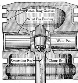
Figure 75.—Piston and Wrist Pin Construction.
