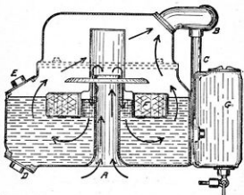
Figure 132.—Air Washer. A—Intake, B—Main Supply Pipe, C—Primary Supply, D—Drain, E—Filler, F—Float, G—Gasoline Tank.
