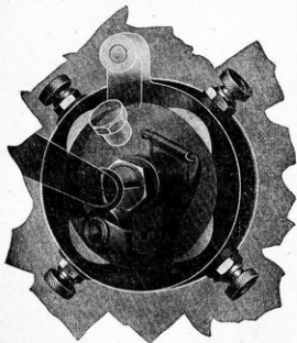
Figure 18.—The Ignition Commutator.
