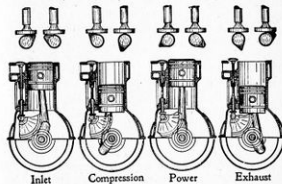
Figure 4.—Piston and Cam Position at Beginning of Strokes.
