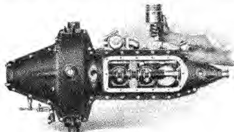
All four pistons may be removed if necessary
