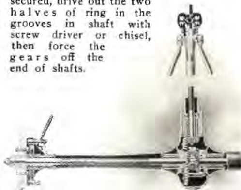
Semi-Sectional View of Rear Axle
