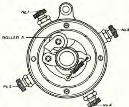
Roller "A" should be on Contact Post No. 1 when Cylinder No. 1 is ready to fire
